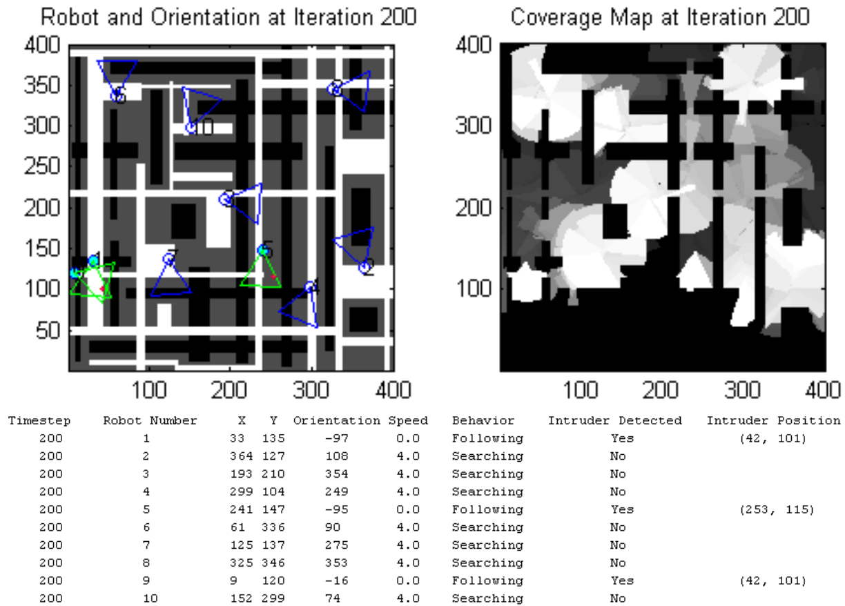
Figure 1: Robot Map and Integrated Coverage Map, together with the Robot Team Status
