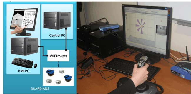
Figure 5: Base station physical setup
